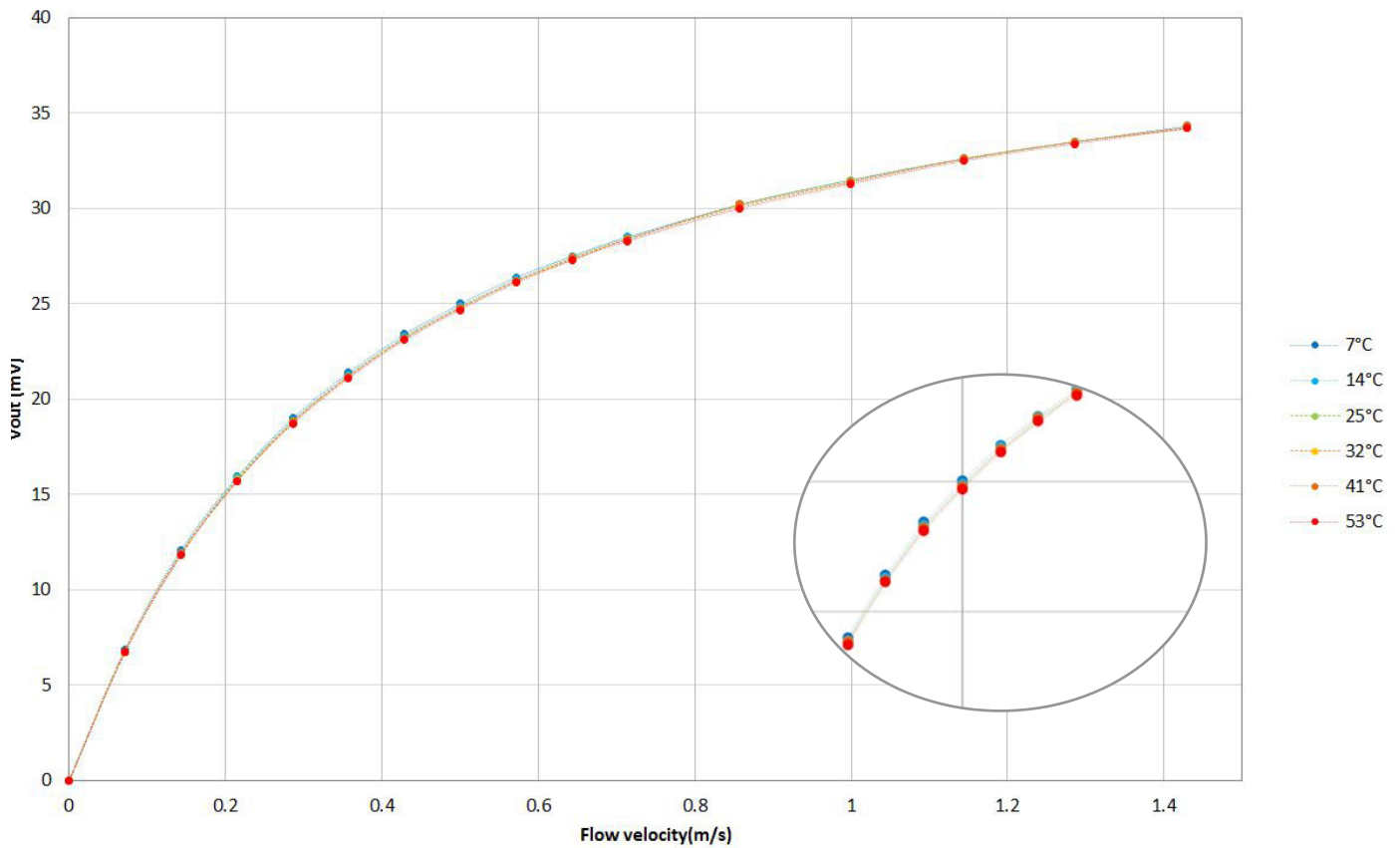
Diagram showing intrinsic temperature compensation
